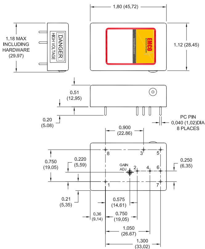
BOTTOM VIEW
